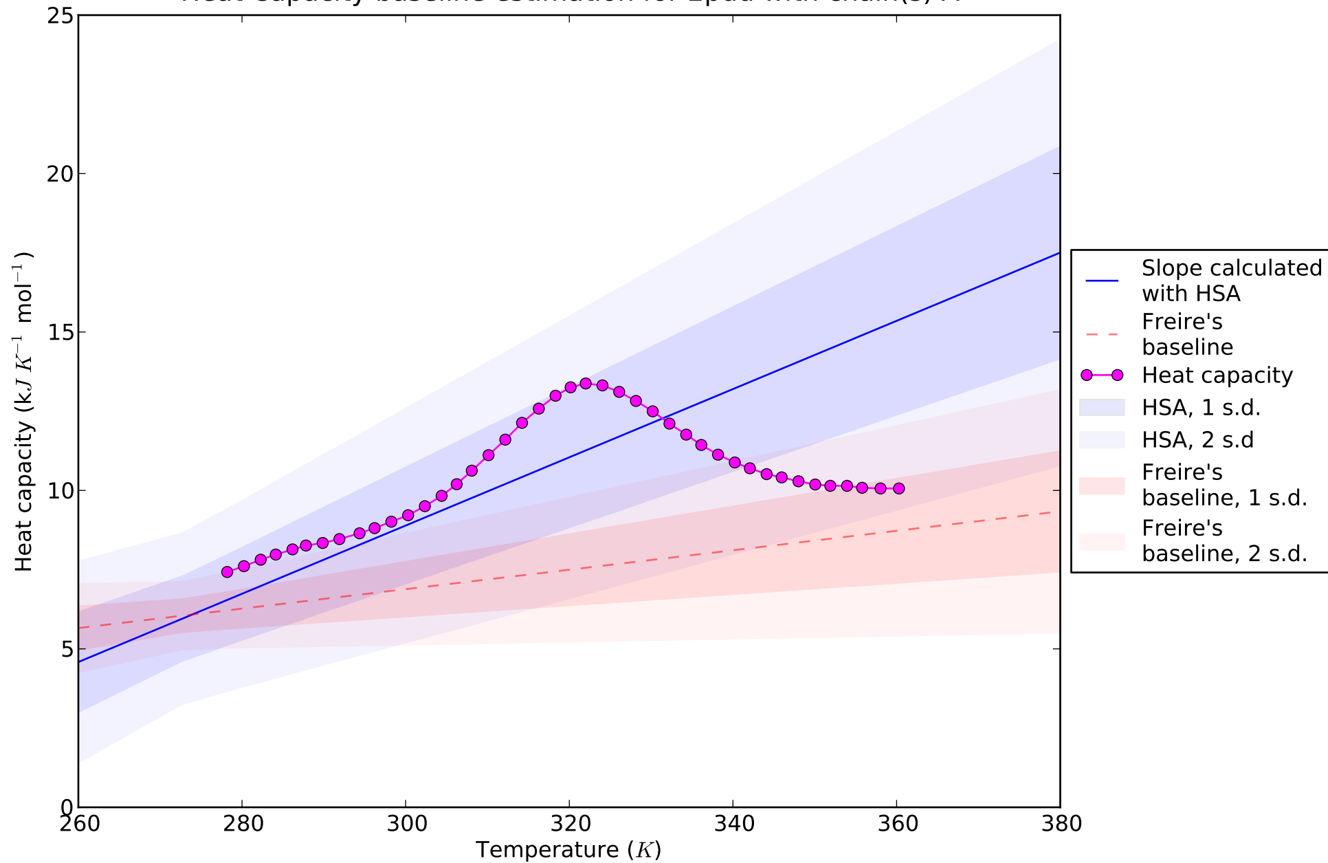
Heat Capacity baseline estimation for 2pdd with chain(s) A
